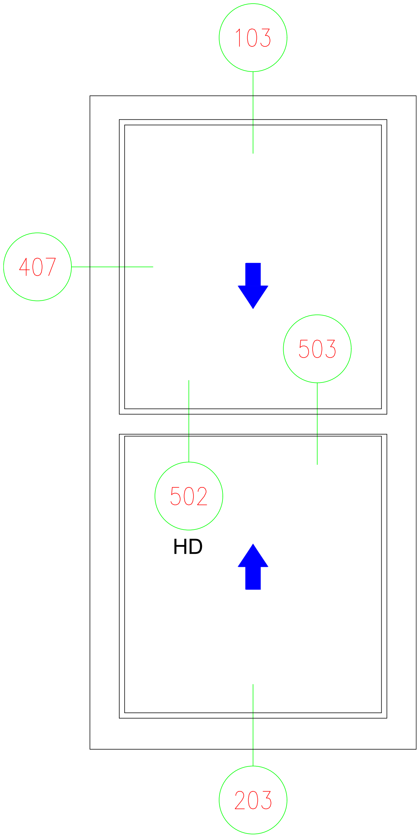
HX45 DOUBLE HUNG INSIDE GLAZED GRID SASH BASE MODEL STANDARD GLAZING
